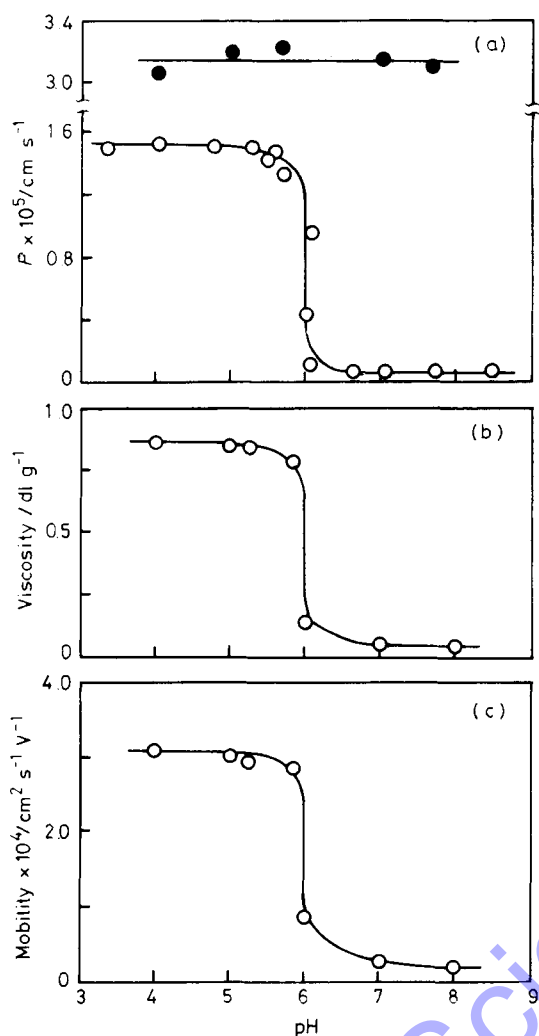
Figure 1. Dependence of P on pH (a) for PSt microcapsules coated with PIE (○) and uncoated (●), and the comparisons of the pH curves with those 7 of intrinsic viscosity (b) and limiting mobility (c) for PIE. The viscosity and mobility were measured at 25 °C using phosphate or acetate buffer adjusted to ionic strength 0.1.
