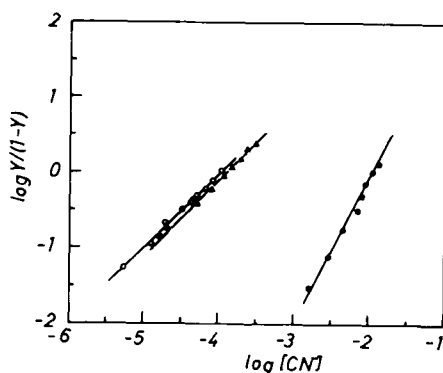
Fig. 6. Hill plots for bovine methemoglobin (○), KPVS-Hb-PDDA complex (△), and hemin (●) at pH 11.97–12.06. Concentration of heme: 6.52 \times 10^{-5} mol/L for methemoglobin; 2.14 \times 10^{-4} for KPVS-Hb-PDDA complex; 8.40 \times 10^{-5} mol/L for hemin. Concentration of potassium cyanide: 0-1.40 \times 10^{-4} mol/L for methemoglobin; 0-4.28 \times 10^{-4} mol/L for KPVS-Hb-PDDA complex; 0-8.40 \times 10^{-3} mol/L.
