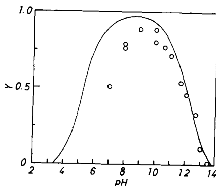
Fig. 5. Curves of Y vs. pH for KPVS-Hb-PDDA complex at C_2/C_1 = 1 ( C_1 = C_2 = 2.14 \times 10^{-4} mol/L): plots, experimental points; full lines, calculation curve by eq. (16).
